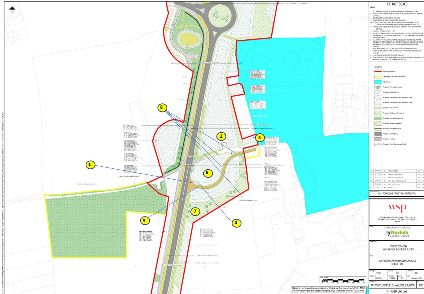
Figure 2-8: Landscape Plan – Sheet 008
