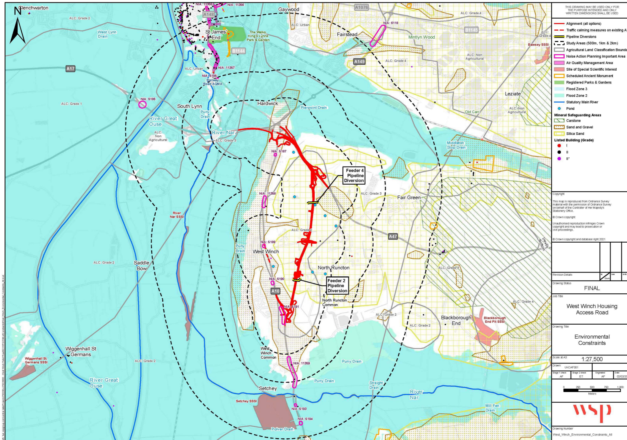
Figure 1.1 – Environmental constraints plan
