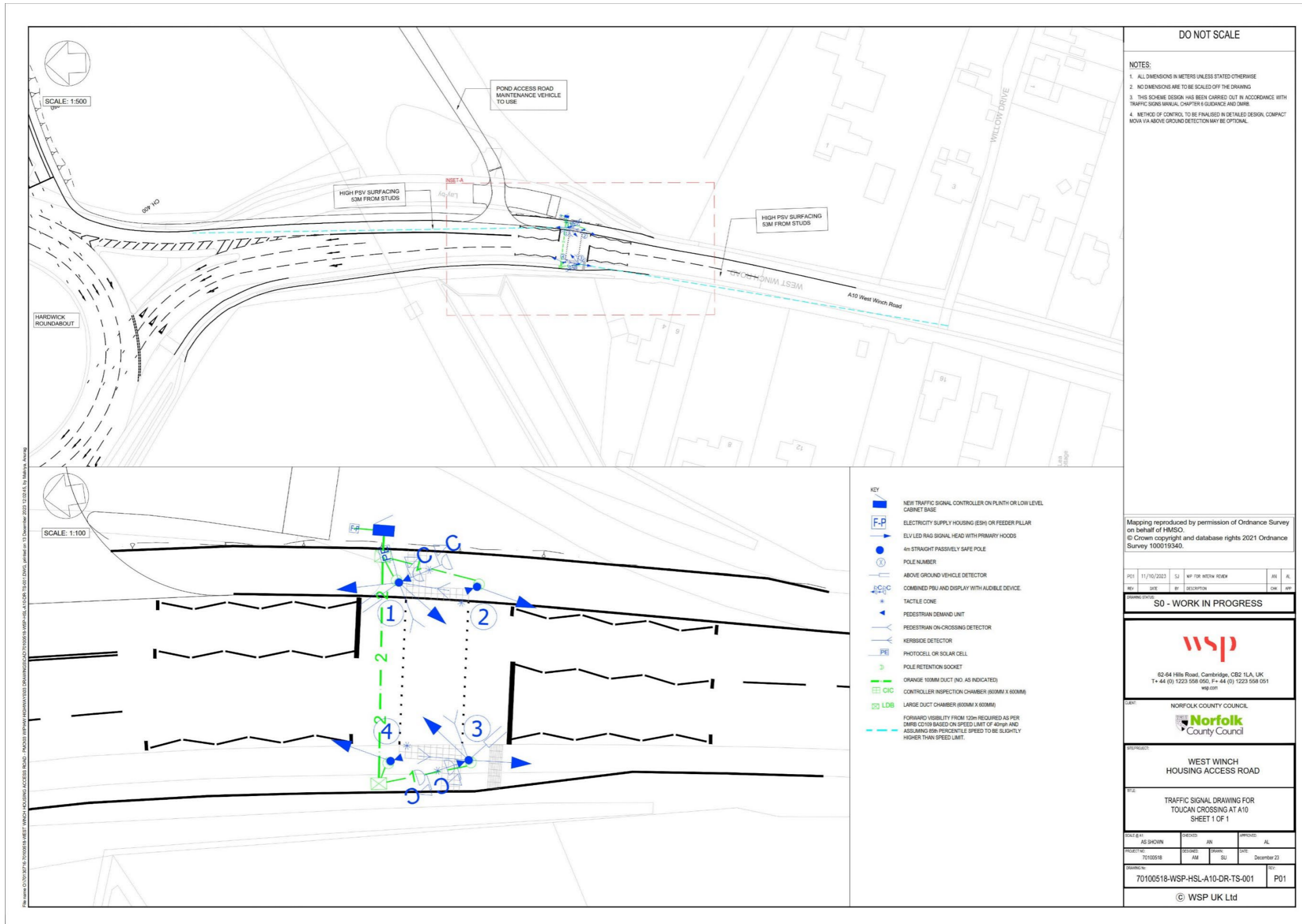
Figure 1-1 – Traffic signal drawing for toucan crossing at A10
