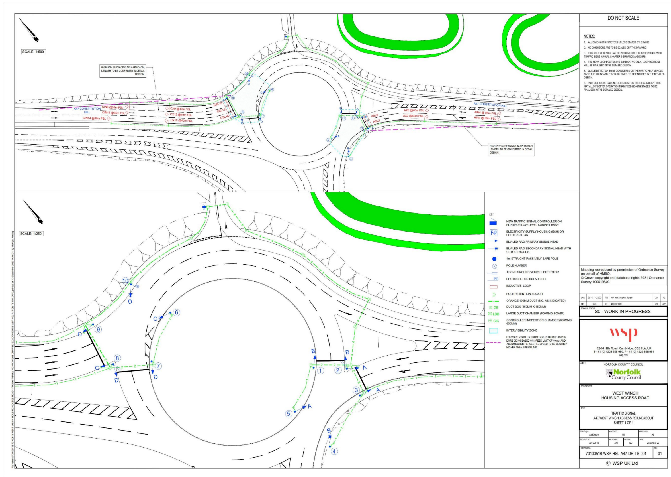
Figure 1-1 – Traffic signal drawing for A47/West Winch access roundabout
