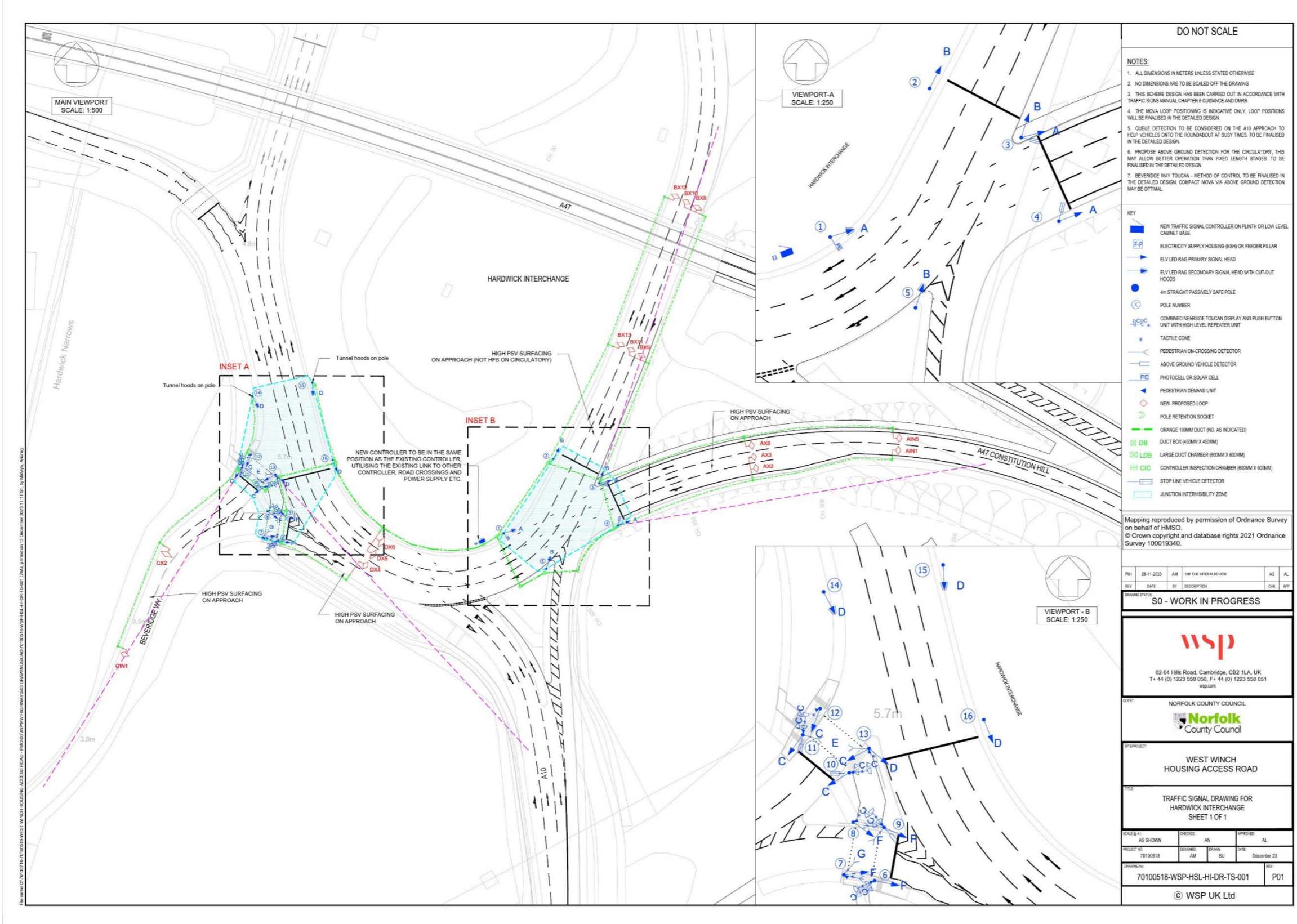
Figure 1-1 – Traffic signal drawing for Hardwick Interchange
