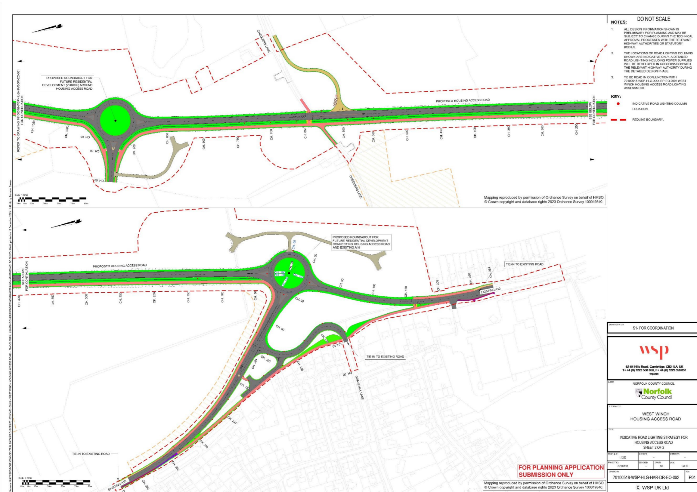
Figure 1-2 - Indicative lighting strategy for housing access road – Sheet 2 of 2
