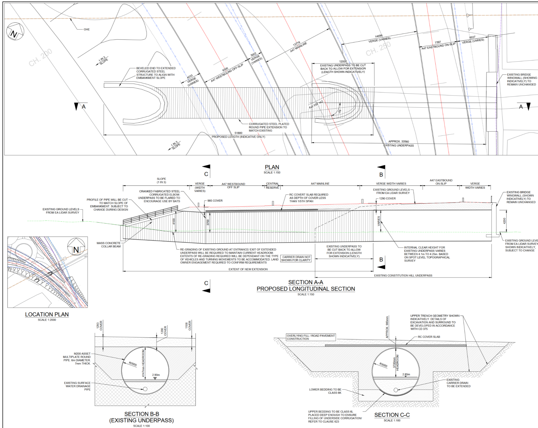
Figure 1 – Constitution Hill Underpass Extension
