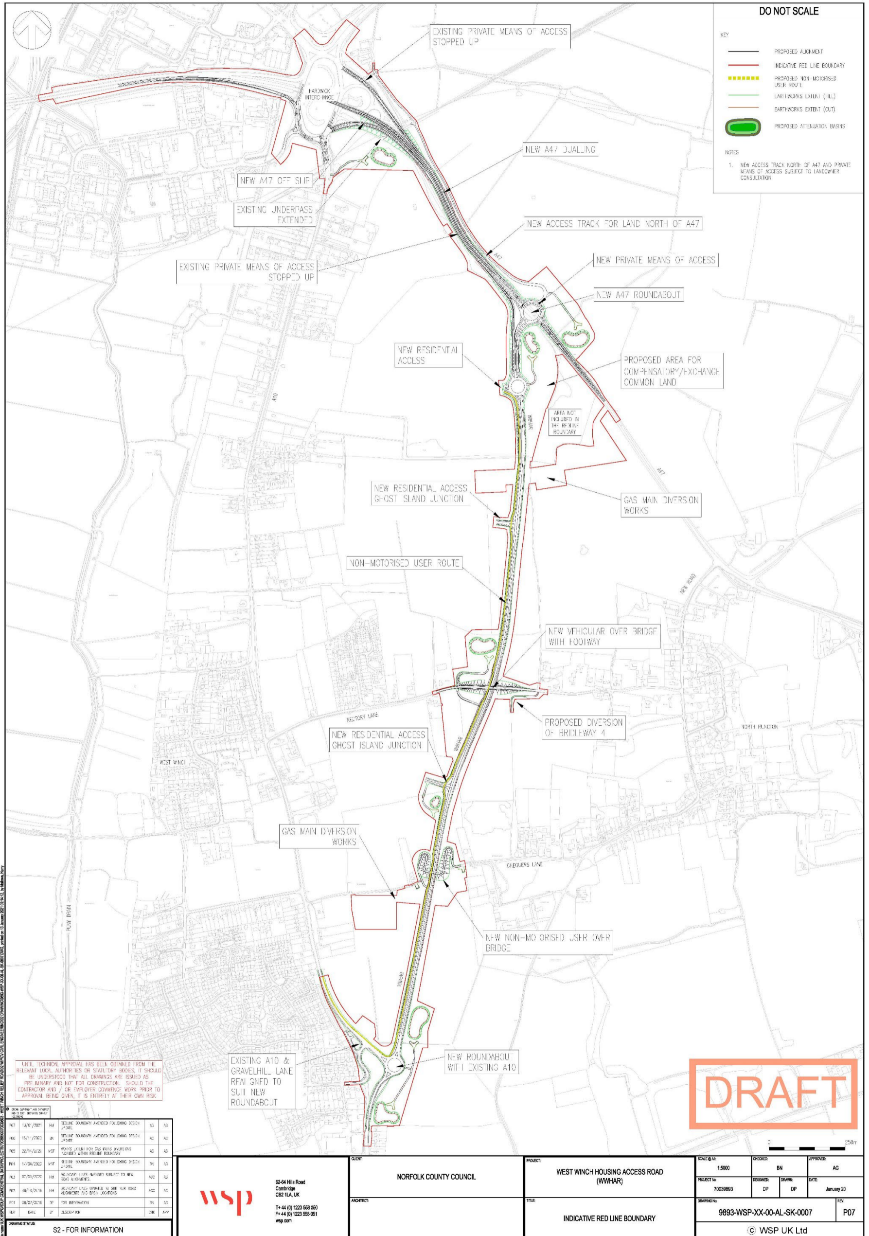
Figure 1.1 – Scheme layout
