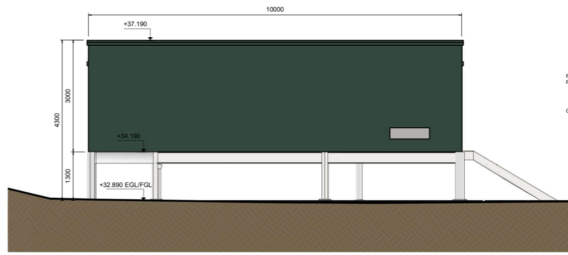
ELEVATION A-A (NORTH) 1 : 50
