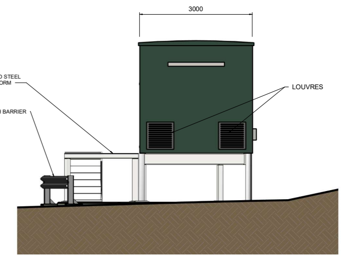
ELEVATION B-B (EAST) 1 : 50
