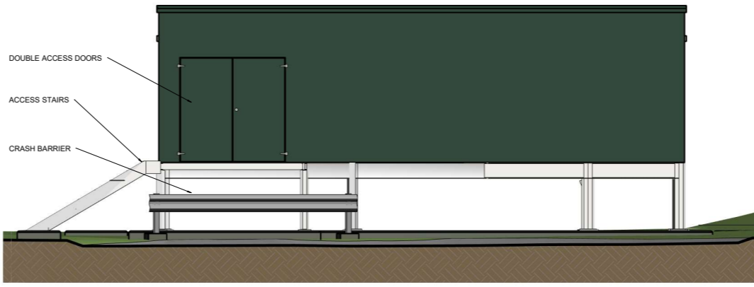
ELEVATION C-C (SOUTH) 1 : 50
