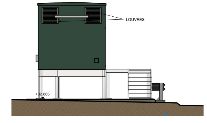
ELEVATION D-D (WEST) 1 : 50
