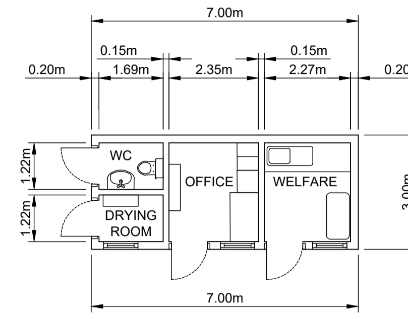
WELFARE UNIT PROPOSED PLAN 1:100@ A1
