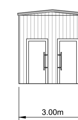
WELFARE UNIT SOUTH ELEVATION 1:100@ A1
