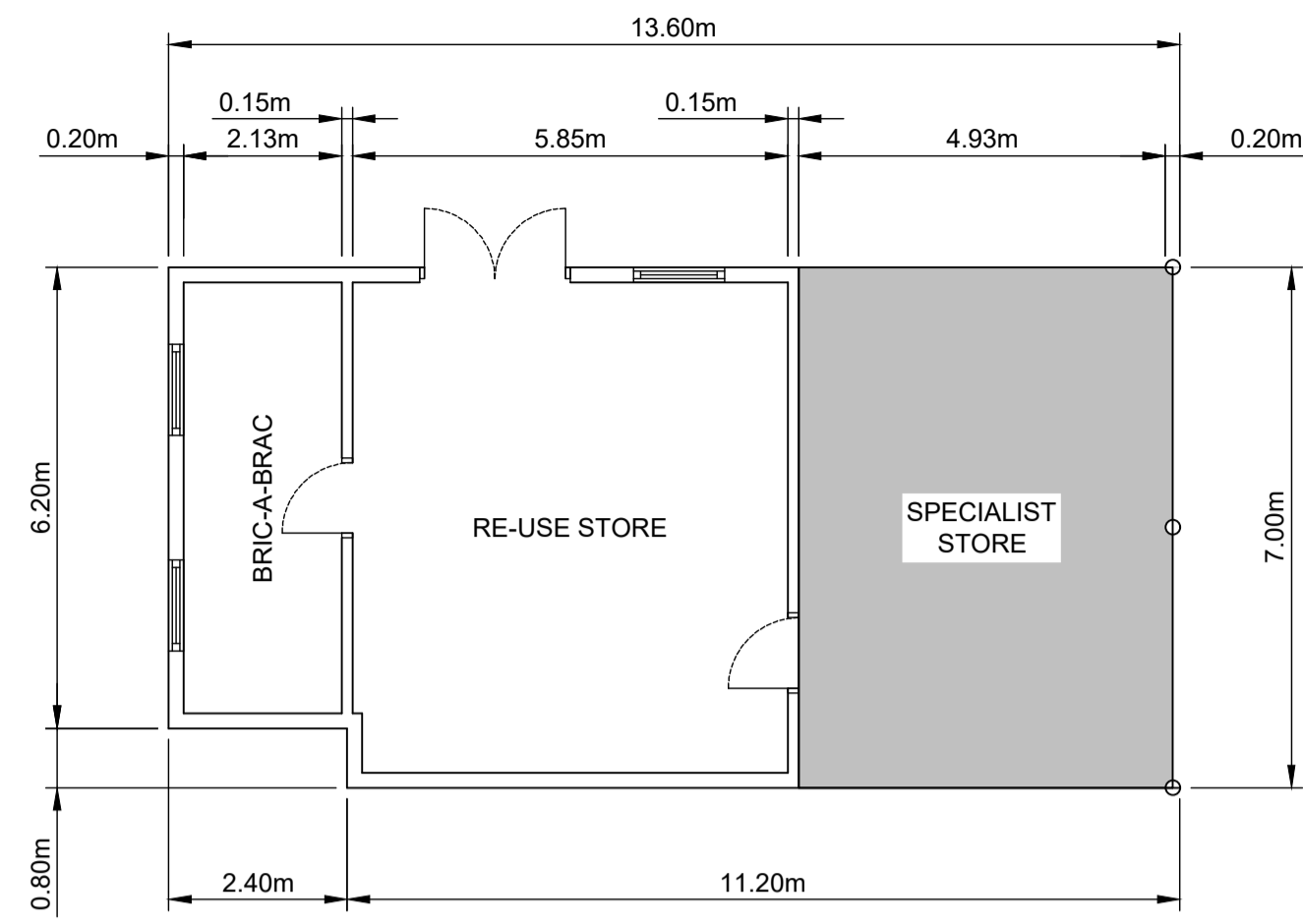
RE-USE STORE PROPOSED PLAN 1:100@ A1
