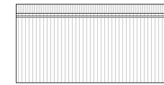
WELFARE UNIT WEST ELEVATION 1:100@ A1
