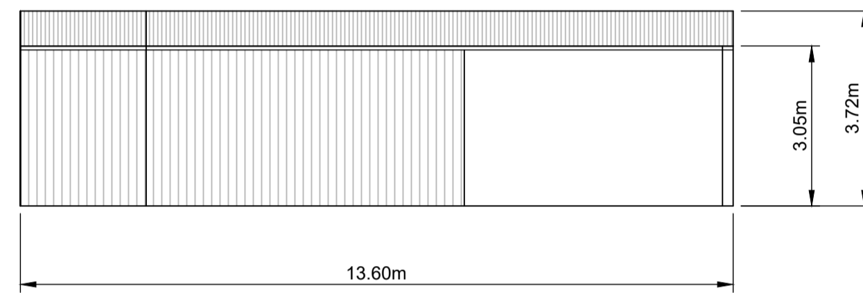
RE-USE STORE NORTH ELEVATION 1:100@ A1
