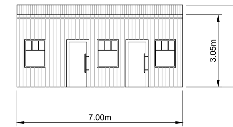
WELFARE UNIT EAST ELEVATION 1:100@ A1
