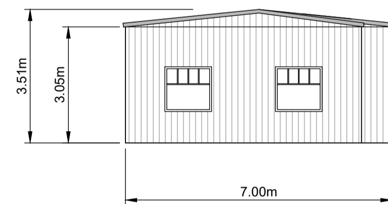
RE-USE STORE EAST ELEVATION 1:100@ A1
