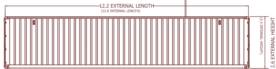
SIDE ELEVATION "A"
