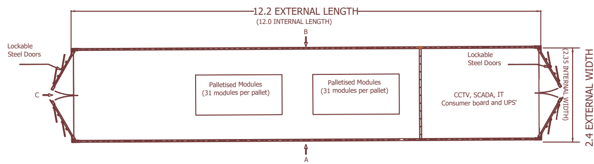
SECTIONAL PLAN
