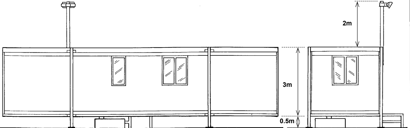
REAR ELEVATION
